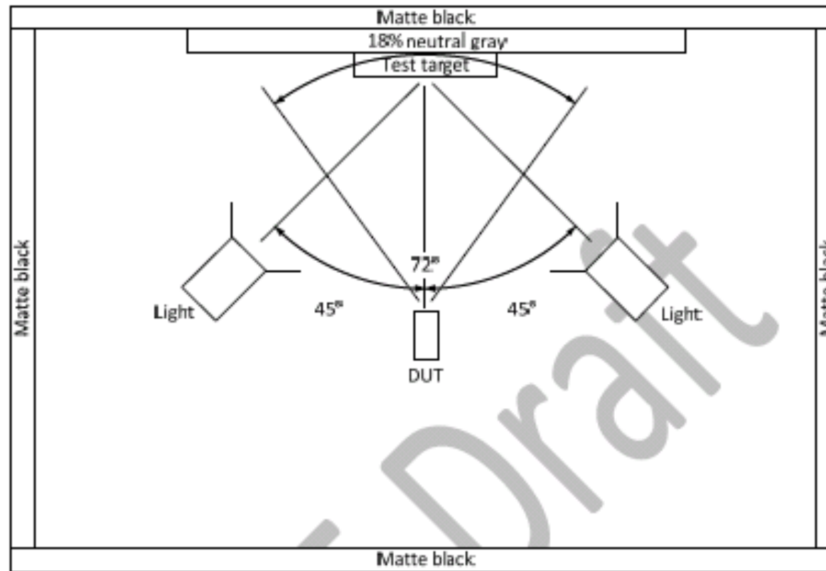
Figure 46: DUT test configuration Ver.:1.02 rev.2
